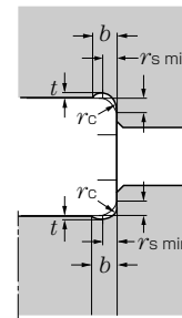
2.12 Relief dimensions for grounding
