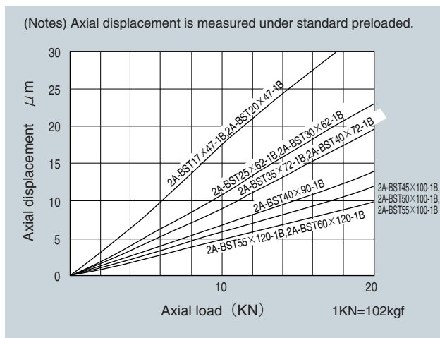
Fig. 13.14 BST type rigidity chart
