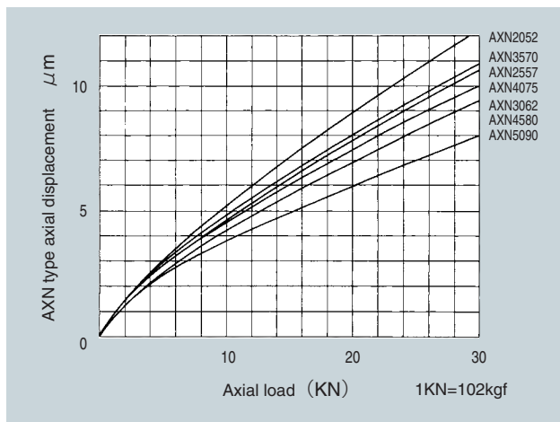
Fig. 13.15 AXN type rigidity chart
