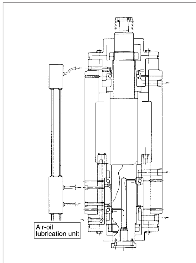
Fig. 9.15 Test rig for measuring temperature rise
