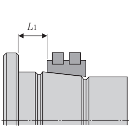
Fig. 6.18 Measurement of bearing position
