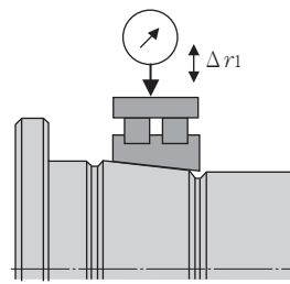
Fig. 6.19 Measurement of bearing radial clearance
