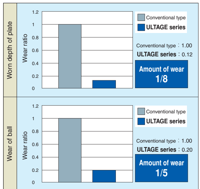
Fig. 13.4 Ratio of fretting corrosion in sliding mode
