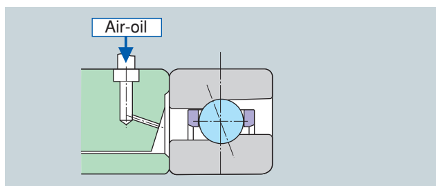
Fig. 8.7 Standard nozzle
