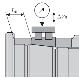
Fig. 6.20 Clearance measurement after insertion of spacer
